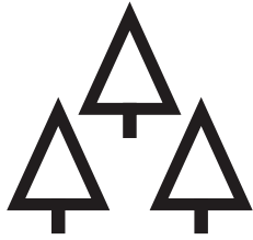
Trees trees.eps
